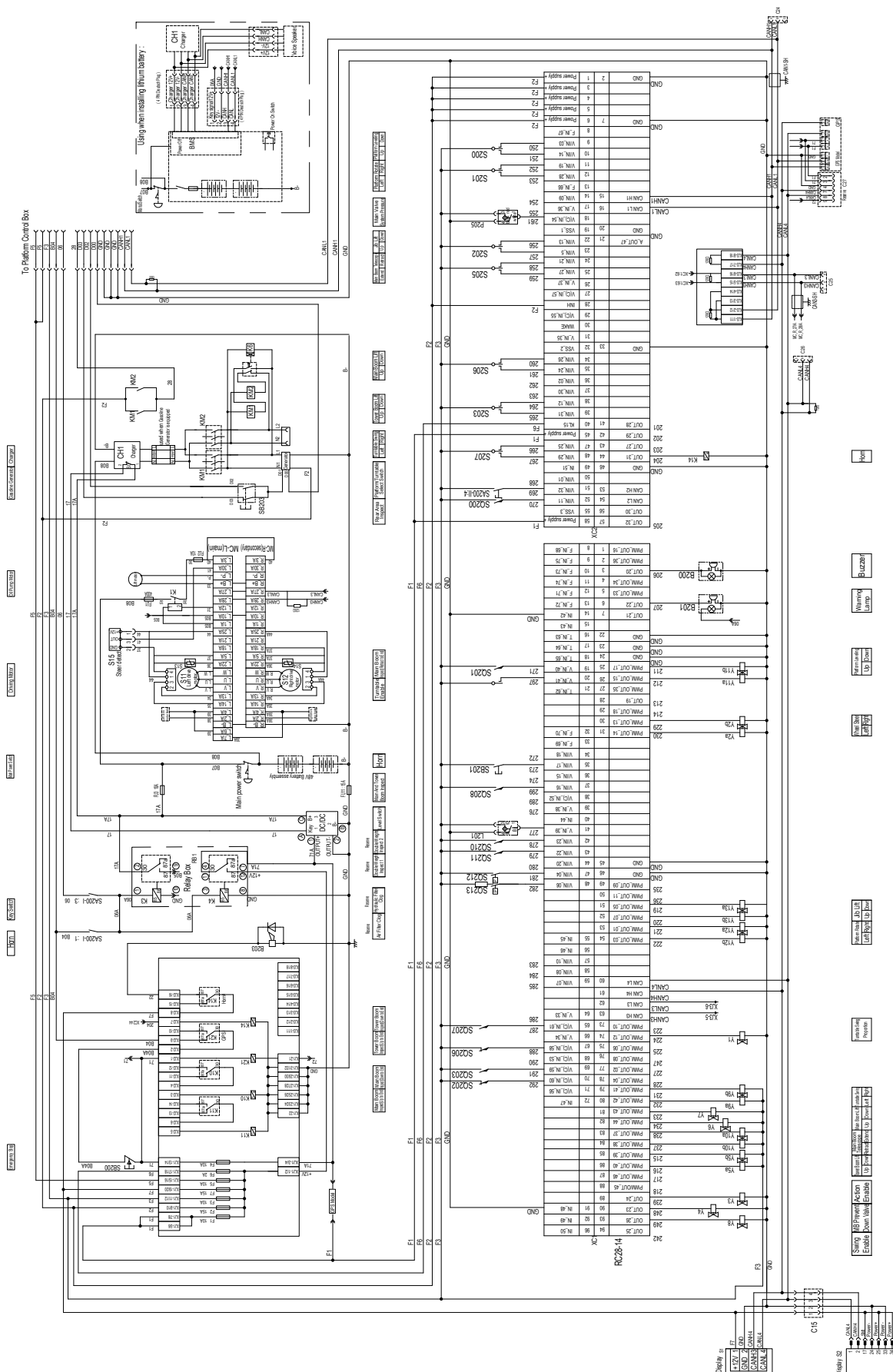
Electrical schematic diagram of turntable (PN.103006060013)
